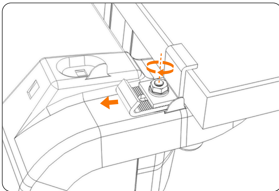
Fig. 9 Module Attachment
