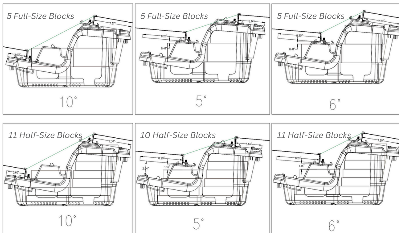
Fig. 28 Full and Half Size Ballast Block Arrangements
