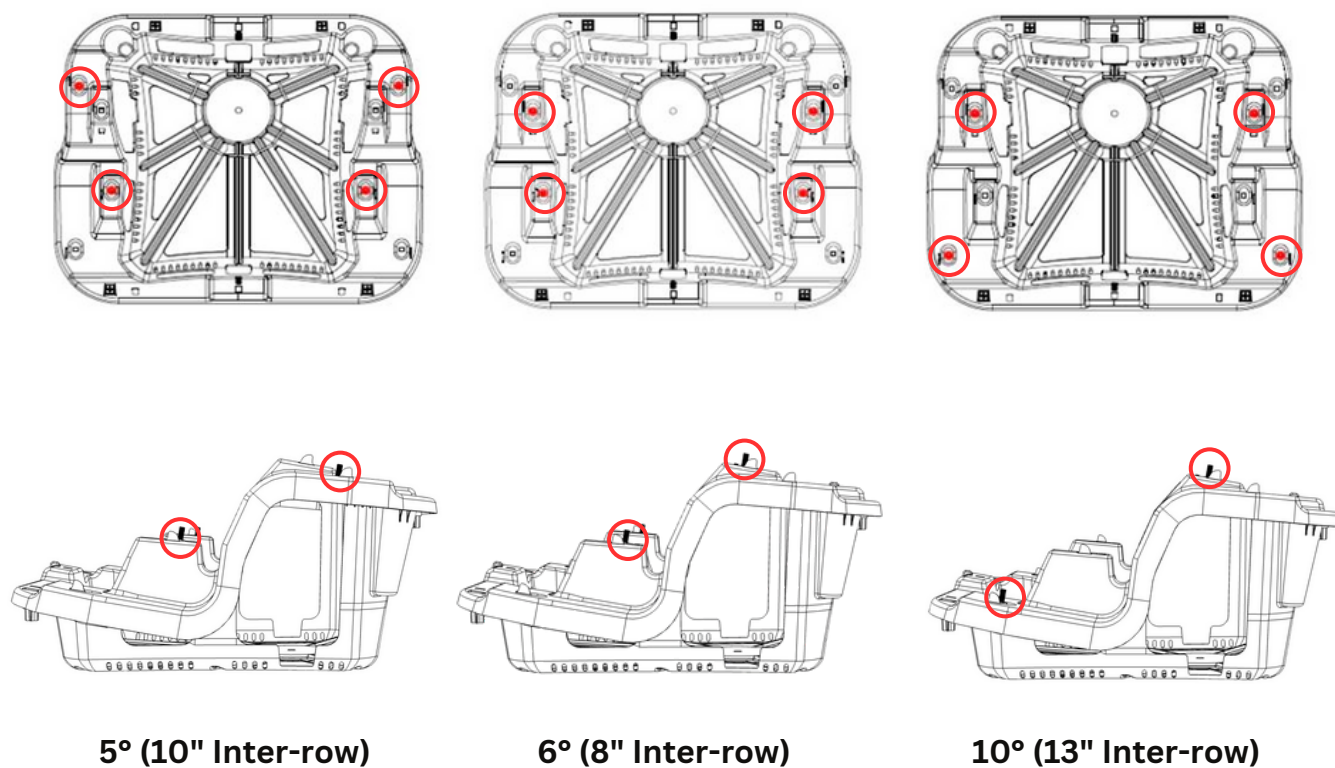
Fig. 2 FR510-6 Pre-Installed Bolt Locations
