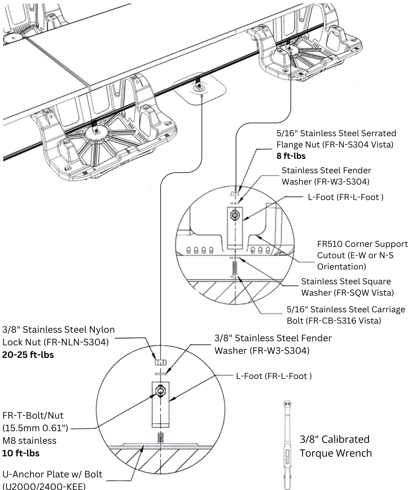
Fig. 13 Mechanical Anchor Installation
